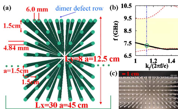
FIG. 2. (Color online) (a) The PC design under study. (b) Surface band and full band gap (shaded region) of the bulk PC are also indicated. The Plexiglas prism fixes the lateral wave vector k_{||} (dot-dashed vertical line) and so excites the mode indicated with the open circle. (c) Picture (top view) of the real PC structure.
