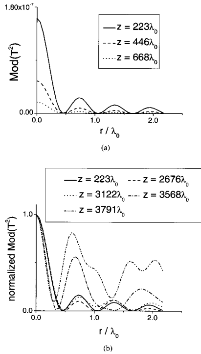
Fig. 8. (a) Transmitted intensity as a function of radial distance for a DBR with \text{TiO}_2/\text{SiO}_2 Bragg reflectors. (b) Normalized transmitted intensity as a function of radial distance for a DBR with \text{TiO}_2/\text{SiO}_2 Bragg reflectors.
