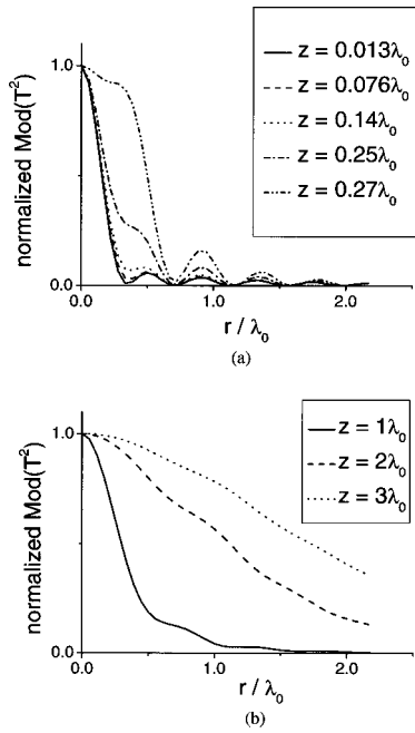
Fig. 12. (a) Normalized transmitted intensity as a function of radial distance for thin film with \epsilon_f = 1.96 + 0.0001i and d_f = 0.357\lambda_0 for fixed z values up to z = 0.27\lambda_0 . (b) Normalized transmitted intensity as a function of radial distance for thin film with \epsilon_f = 1.96 + 0.0001i and d_f = 0.357\lambda_0 for fixed z values up to z = 3\lambda_0 .
